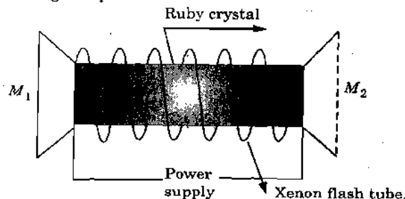
Fig. 5.22.1. Construction of Ruby laser.
