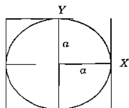
Fig. 1. (c) Circularly polarized light.
