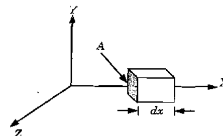
Fig. 2.9.1. Illustration of concept of poynting vector.
