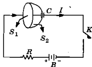
Fig. 2.7.1. Electric circuit showing the concept of displacement current.
