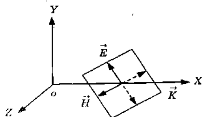
Fig. 2.15.1. Transverse nature of EM-waves in free space (or vacuum).
