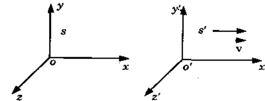
Fig. 1.2.1: Galilean transformation
