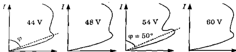
Fig. 2. Plots of intensity of electron beam against scattering angle for different values of accelerating voltage.
