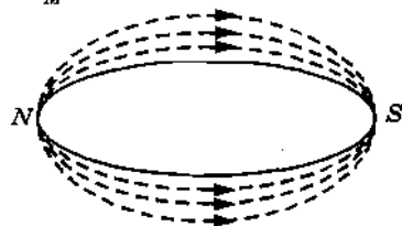
Fig. 2.3.2. Magnetic flux through a closed surface
