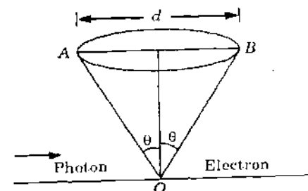
Fig. 3. Measurement of position and linear momentum of an electron.
