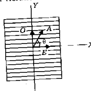
Fig. 1. Double refraction in a uniaxial crystal.
