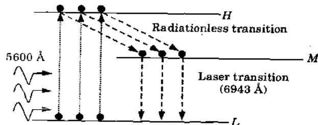
Fig. 5.22.2. Energy level diagram of Ruby laser.
