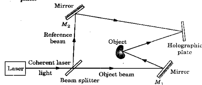
Fig. 5. Recording of hologram.
