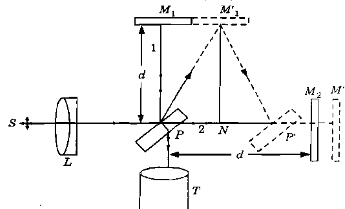
Fig. 1.4.1 The Michelson-Morley experiment.
