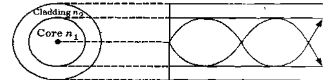
Fig. 5.4.4. Propagation in a multimode graded index fibre.
