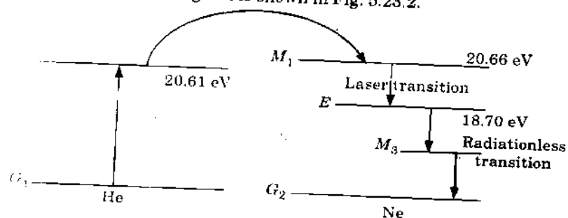
Fig. 5.23.2. Energy level diagram of He-Ne laser.
