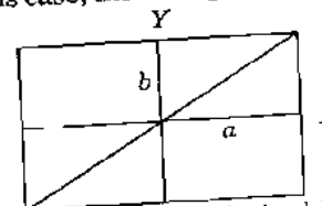
Fig. 1. (a) Plane polarized light.
