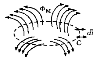
Fig. 2.3.3. Induced emf in a current carrying coil.
