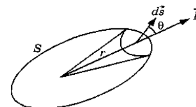
Fig. 2.3.1. A closed surface enclosing charge q .
