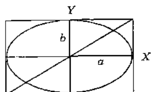
Fig. 1. (b) Elliptically polarized light.
