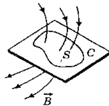
Fig. 2.3.4. A closed current-carrying loop.
