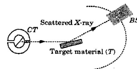
Fig. 3.24.1. Experimental verification of Compton effect.
