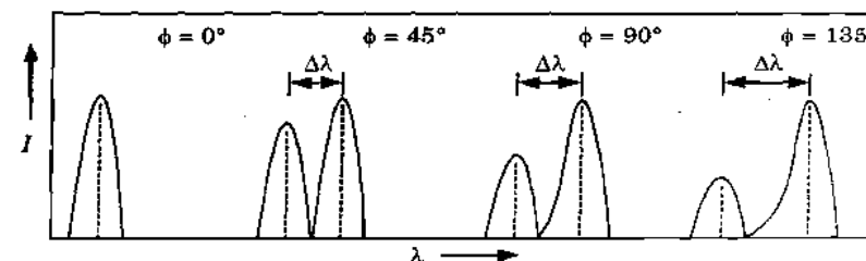
Fig. 3.24.2. Intensity of scattered X-rays.
