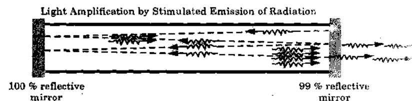
Fig. 5.22.3. Photon multiplication in Ruby laser.
