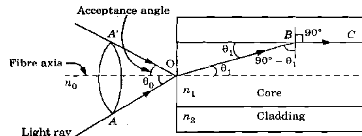
Fig. 5.3.1. Light propagation in an optical fibre.
