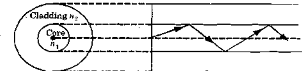
Fig. 5.4.5. Propagation in a single mode step index fibre.
