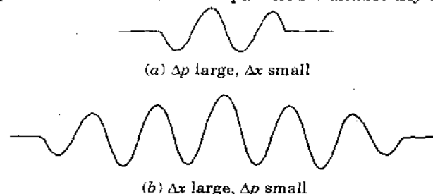
Fig. 2. Wave-packet : (a) Narrow, and (b) Wide.
