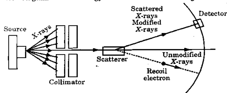
Fig. 3.23.1. Compton effect
