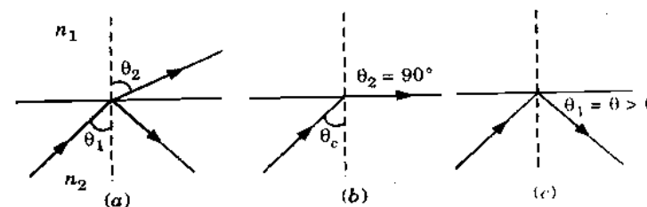
Fig. 5.2.1. Principle of optical fibre.
