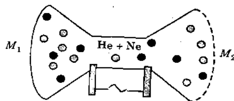
Fig. 5.23.1. Construction of He-Ne laser.
