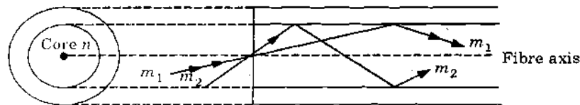
Fig. 5.4.2. Propagation in multimode step index fibre.
