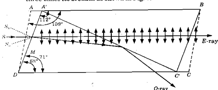
Fig. 4. Construction of a calcite crystal.
