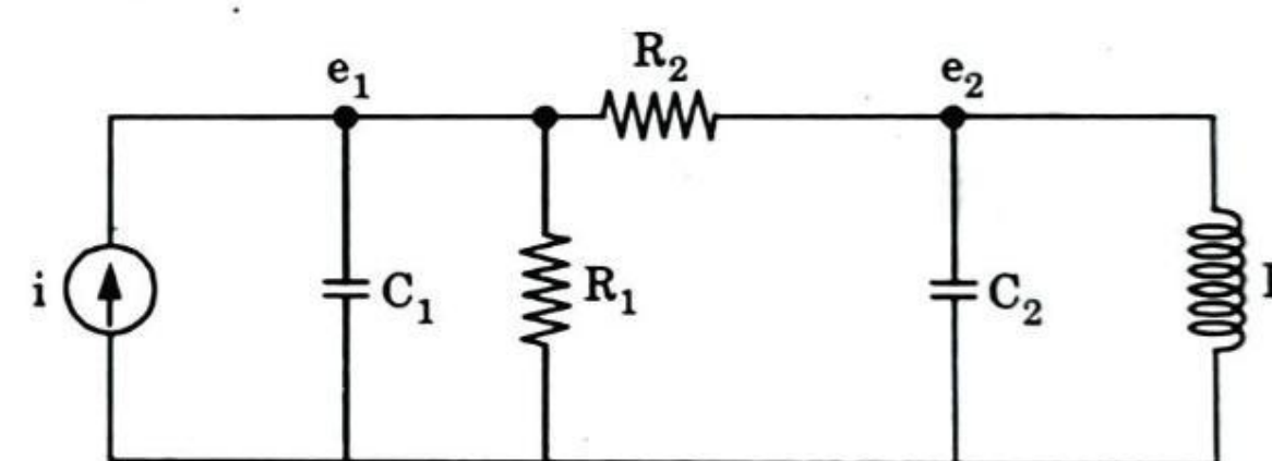
Fig. 1.30.3. Force-current analogous circuit.
