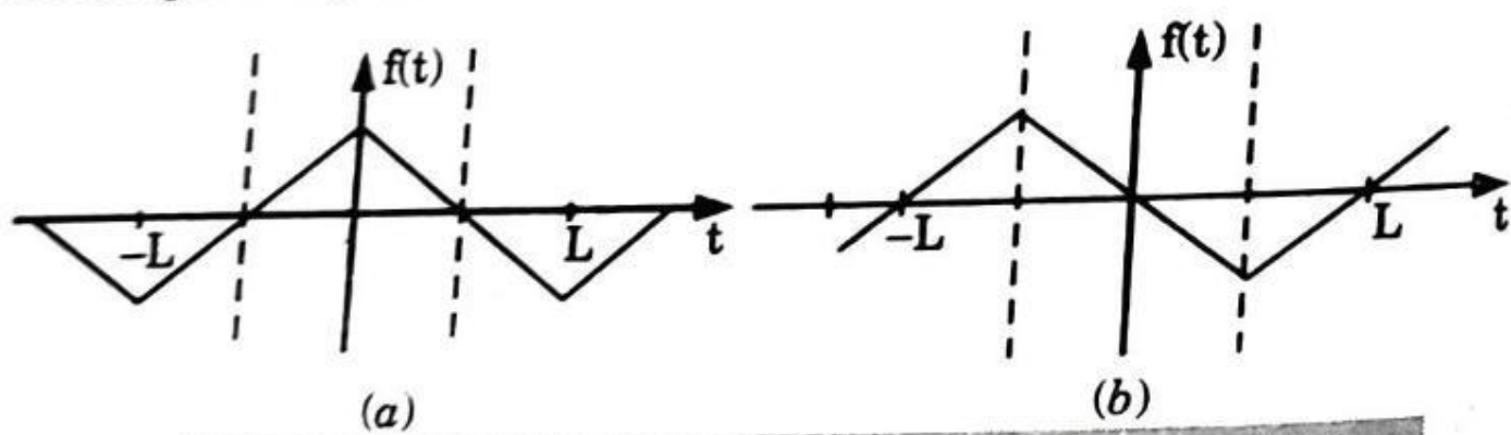
Fig. 2.3.4. (a) Even signal with Quarter wave symmetry. (b) Odd signal with Quarter wave symmetry.
