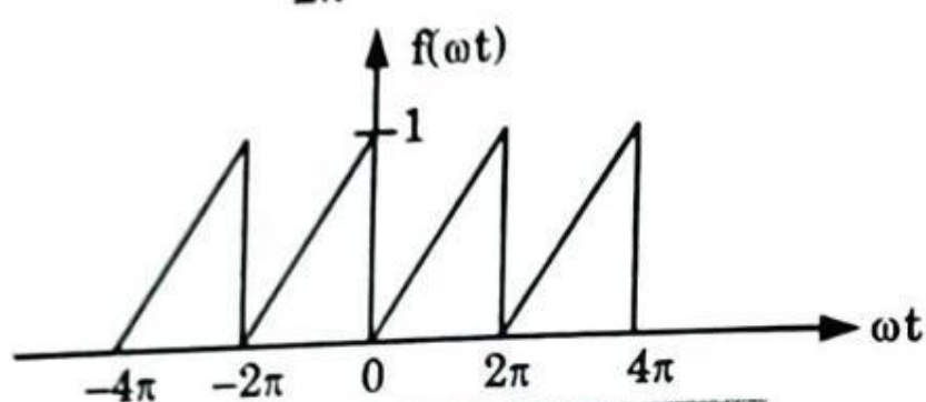
Fig. 2.7.1. Sawtooth wave.
