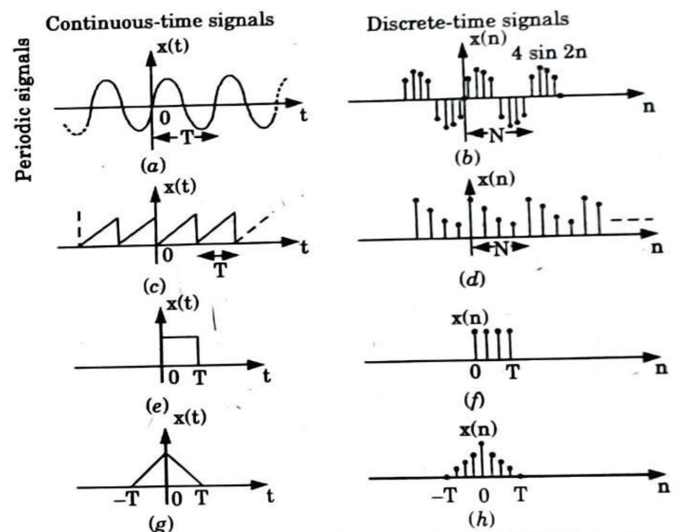
Fig. 1.7.1. (a), (b), (c) and (d) periodic signals; (e), (f), (g) and (h) non-periodic signals.
