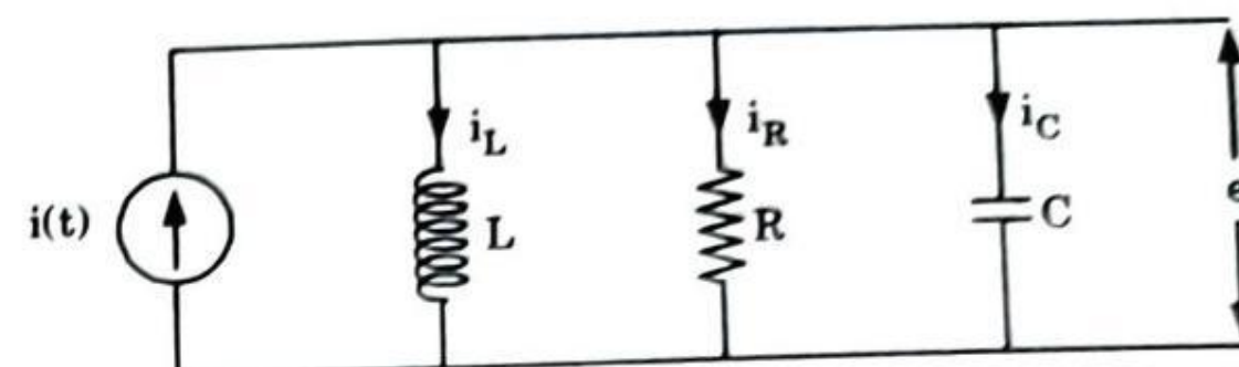
Fig. 1.25.3. Force-current analogous circuit.
