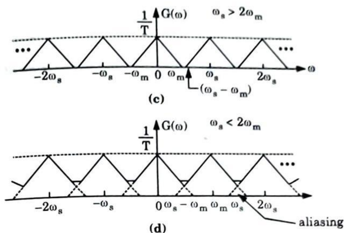
Fig. 2.29.2. Continuous signal, impulse train sampled signal spectrum.
