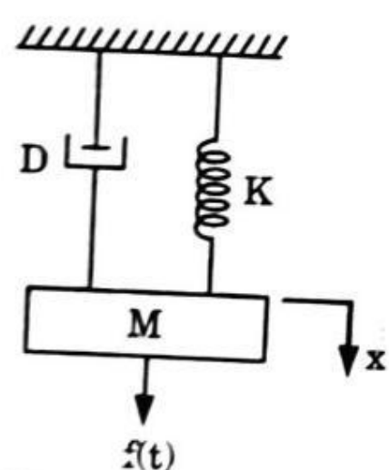
Fig. 1.25.1. Mechanical system.
