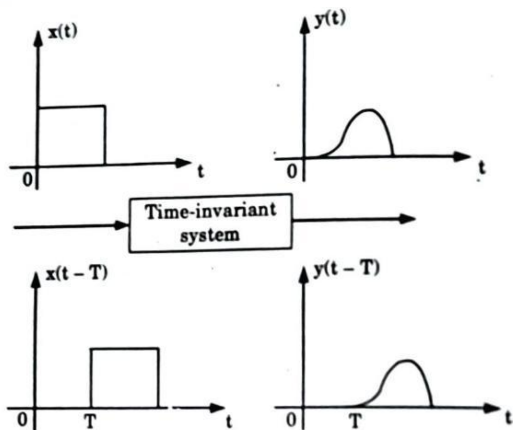
Fig. 1.20.1. Time-invariant system.
