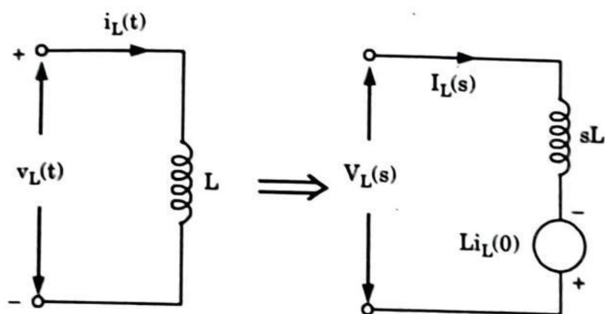
(a) Inductive element
