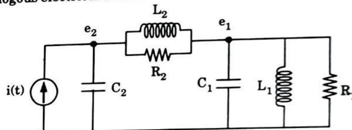
Fig. 1.28.2. Force-current analogous circuit.
