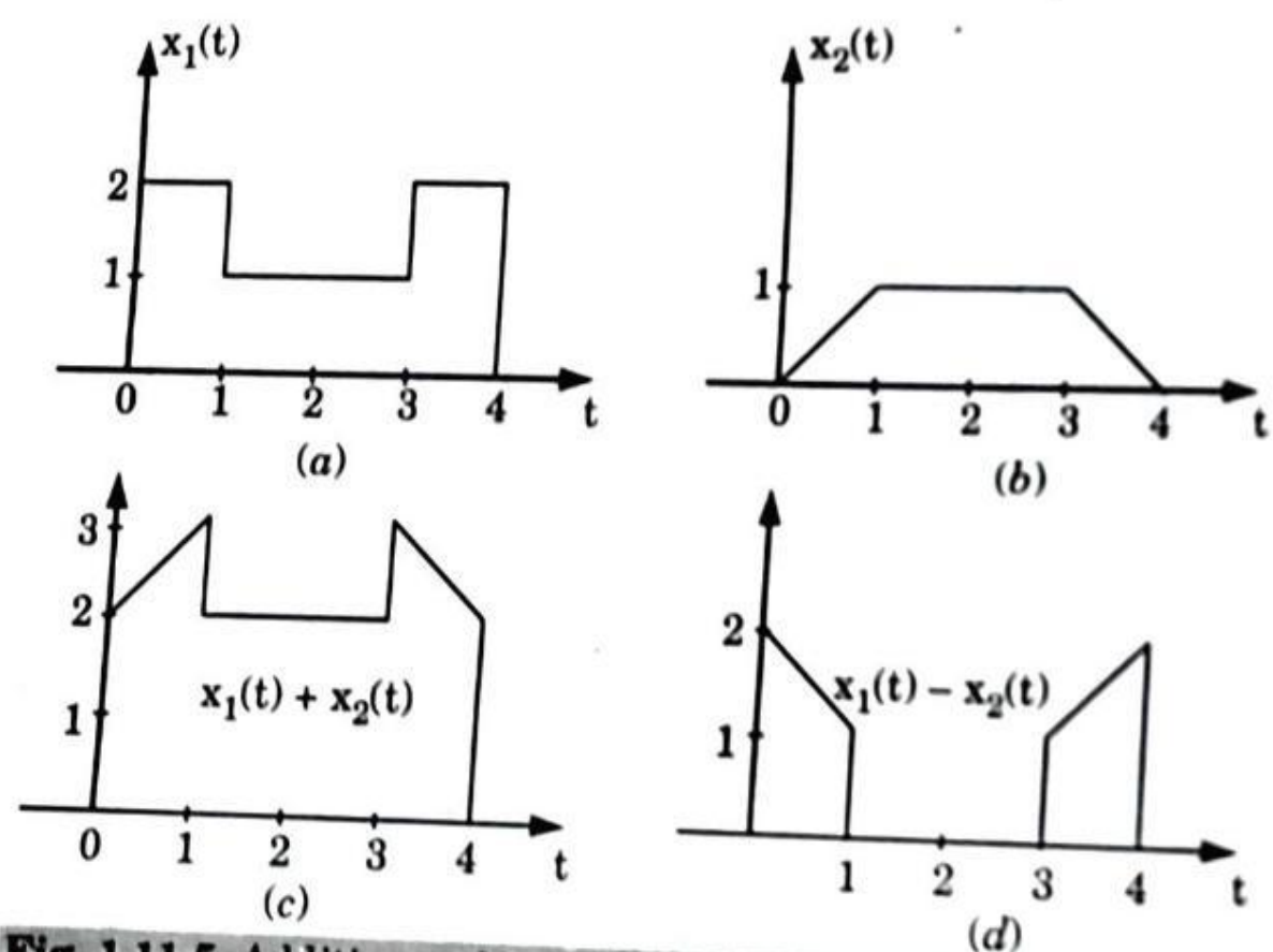
Fig. 1.11.5. Addition and subtraction of continuous-time signals.
