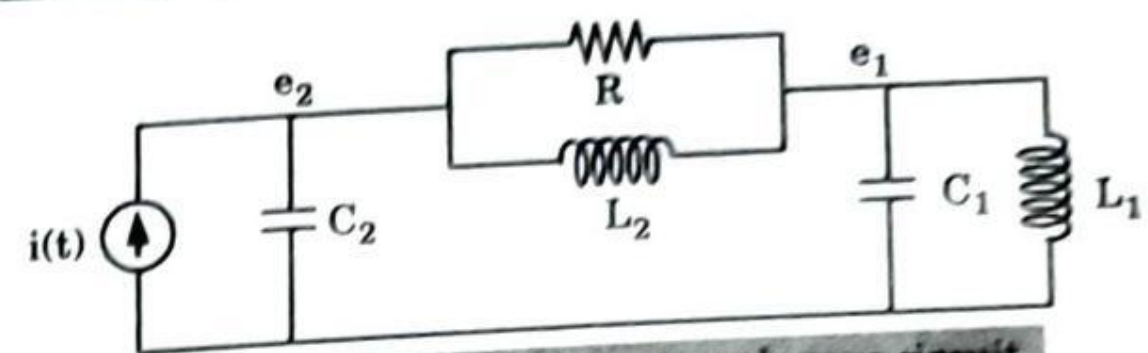
Fig. 1.31.3. Force-current analogous circuit.
