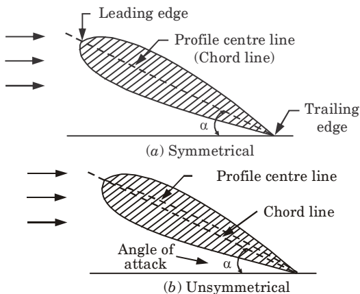
Fig. 3.37.1. Airfoil.
