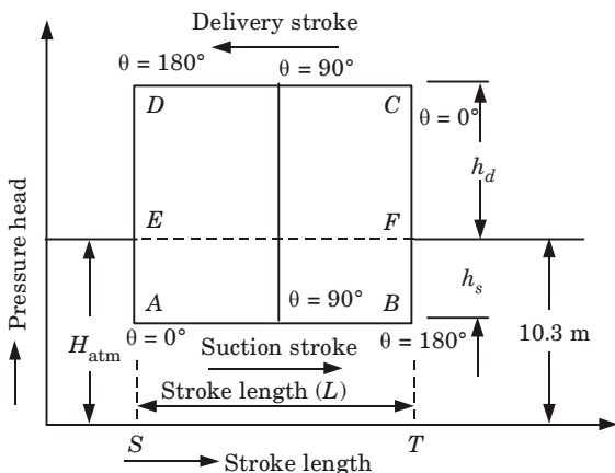
Fig. 5.28.1. Ideal indicator diagram.
