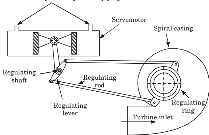
Fig. 4.24.1. Governing of Francis turbine.
