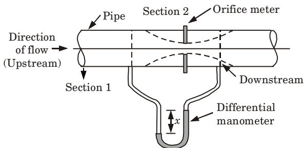
Fig. 1.12.2. Orifice Meter.
