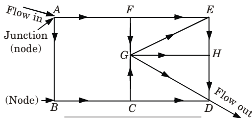
Fig. 3.19.1. Pipe network.
