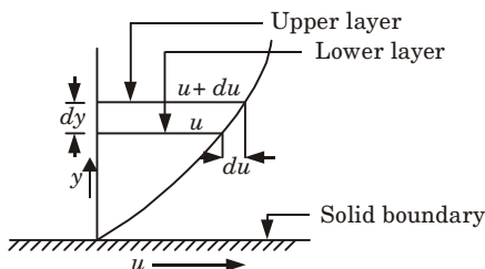
Fig. 1.1.1. Velocity variation near a solid boundary.
