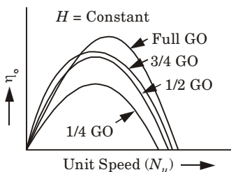
Fig. 4.36.1. Main characteristic curves for a Pelton wheel.
