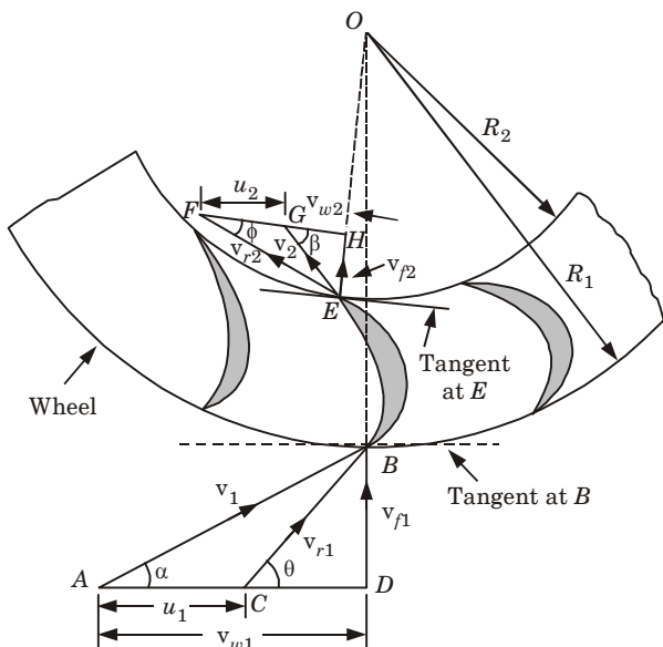
Fig. 4.22.1. Series of radial curved vanes mounted on a wheel.
