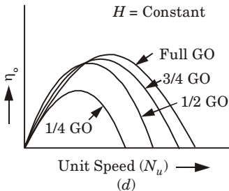
Fig. 4.36.2. Main characteristic curves for reaction turbine.
