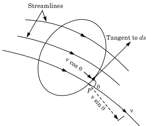
Fig. 2.10.1. Circulation in a two-deimensinal flow.
