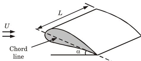
Fig. 3.38.1. Airfoil.
