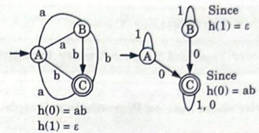
Fig. 2.22.1. Inverse homomorphism construction.
