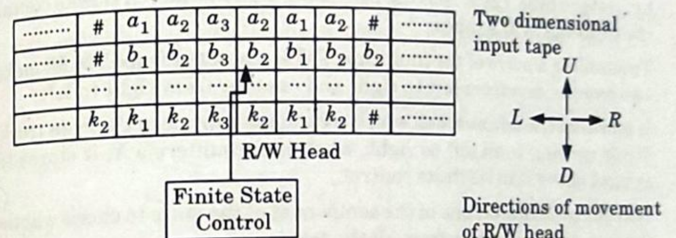
Fig. 5.9.1. A multidimensional Turing machine model.
