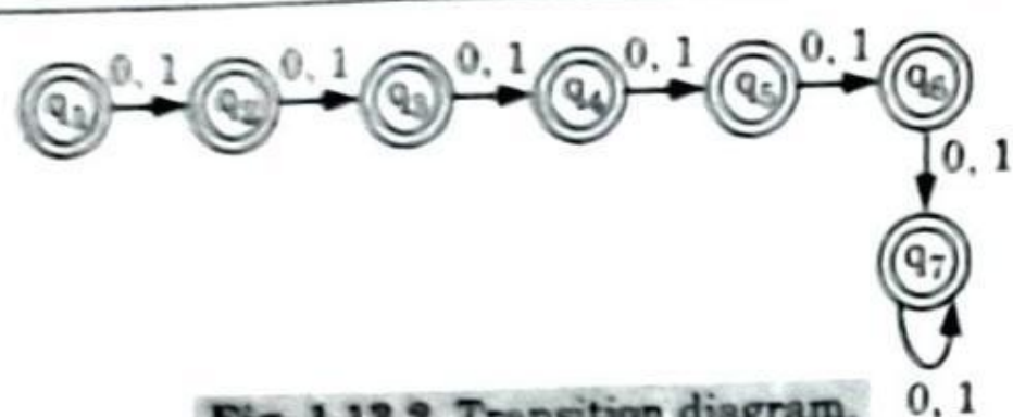
Fig. 1.13.2. Transition diagram.
