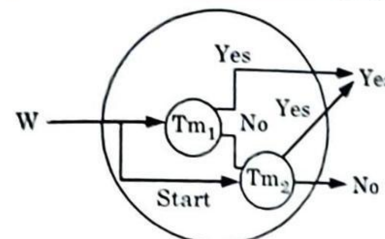
Fig. 5.21.2. Construction for union.
