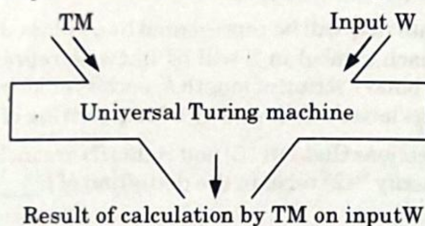
Fig. 5.16.1. Result of calculation by TM on input w .
