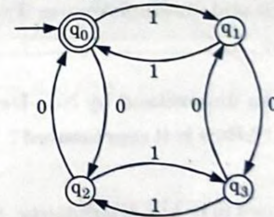
Fig. 1.13.1. Transition diagram.
