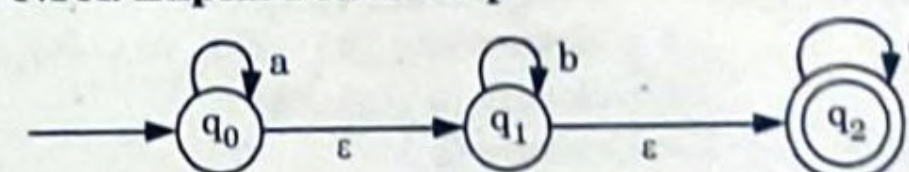
Fig. 1.26.1. NFA with \epsilon -transition ( \epsilon -NFA).
