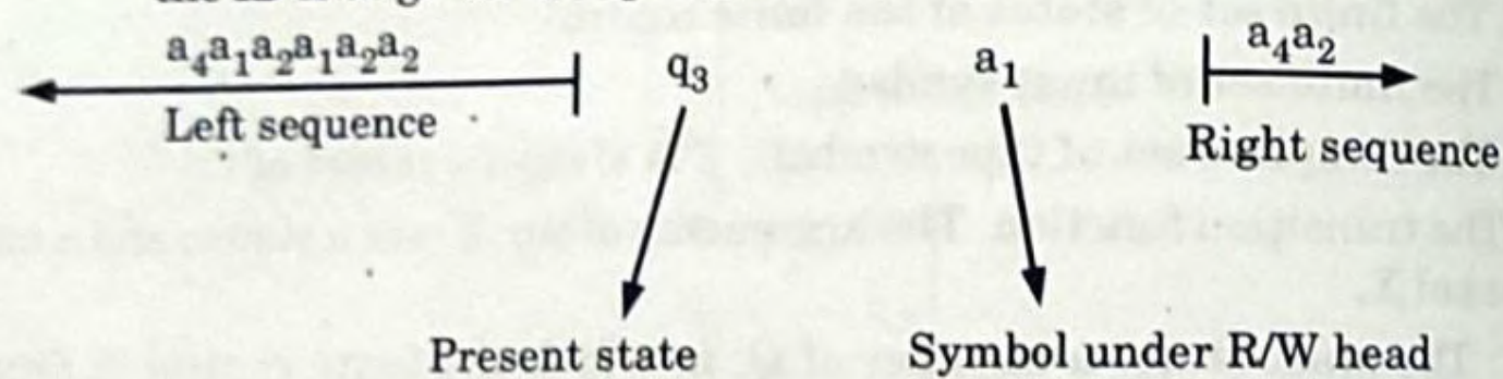
Fig. 5.3.2. Representation of ID.
