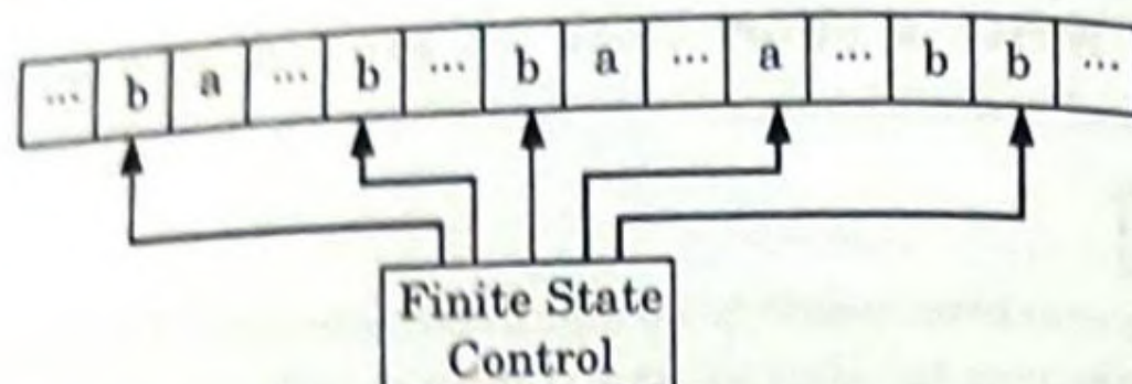
Fig. 5.10.1. A multihead Turing machine model (five heads).
