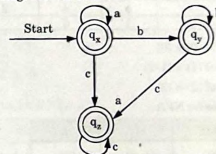
Fig. 1.26.2. NFA without \epsilon -transitions.
