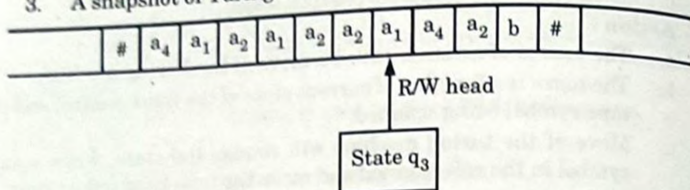
Fig. 5.3.1. A snapshot of Turing machine.
