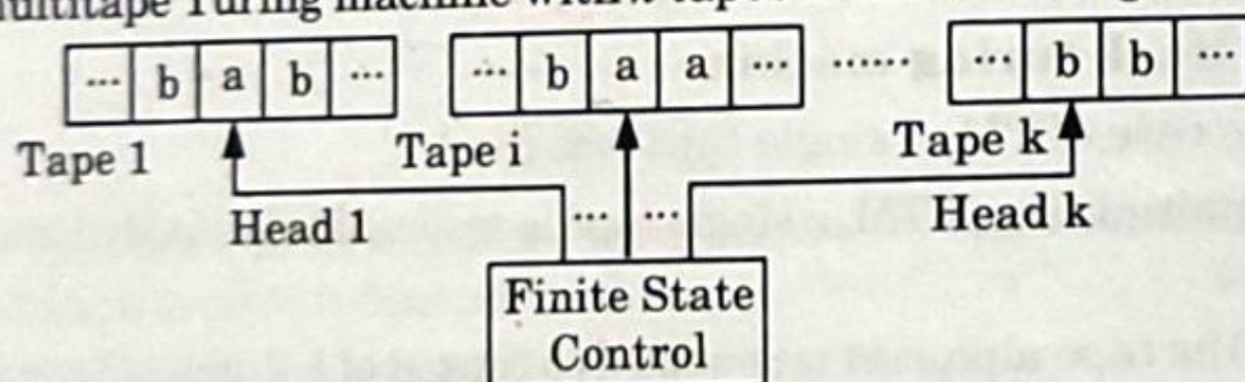
Fig. 5.8.1. A multitape Turing machine model.
