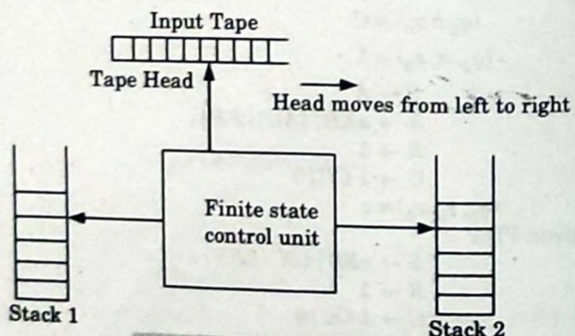
Fig. 4.24.1. Two stack PDA.
