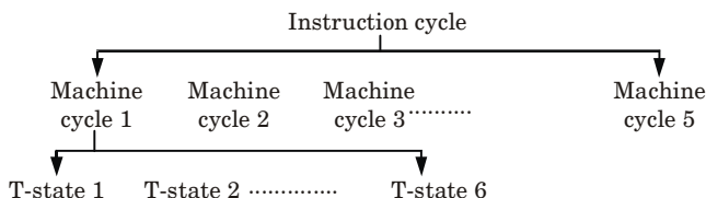
Fig. 1.16.2. Relationship between instruction cycle, machine cycle and T-state.
