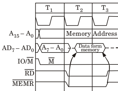
Fig. 1.20.2. Timing diagram of memory read cycle.
